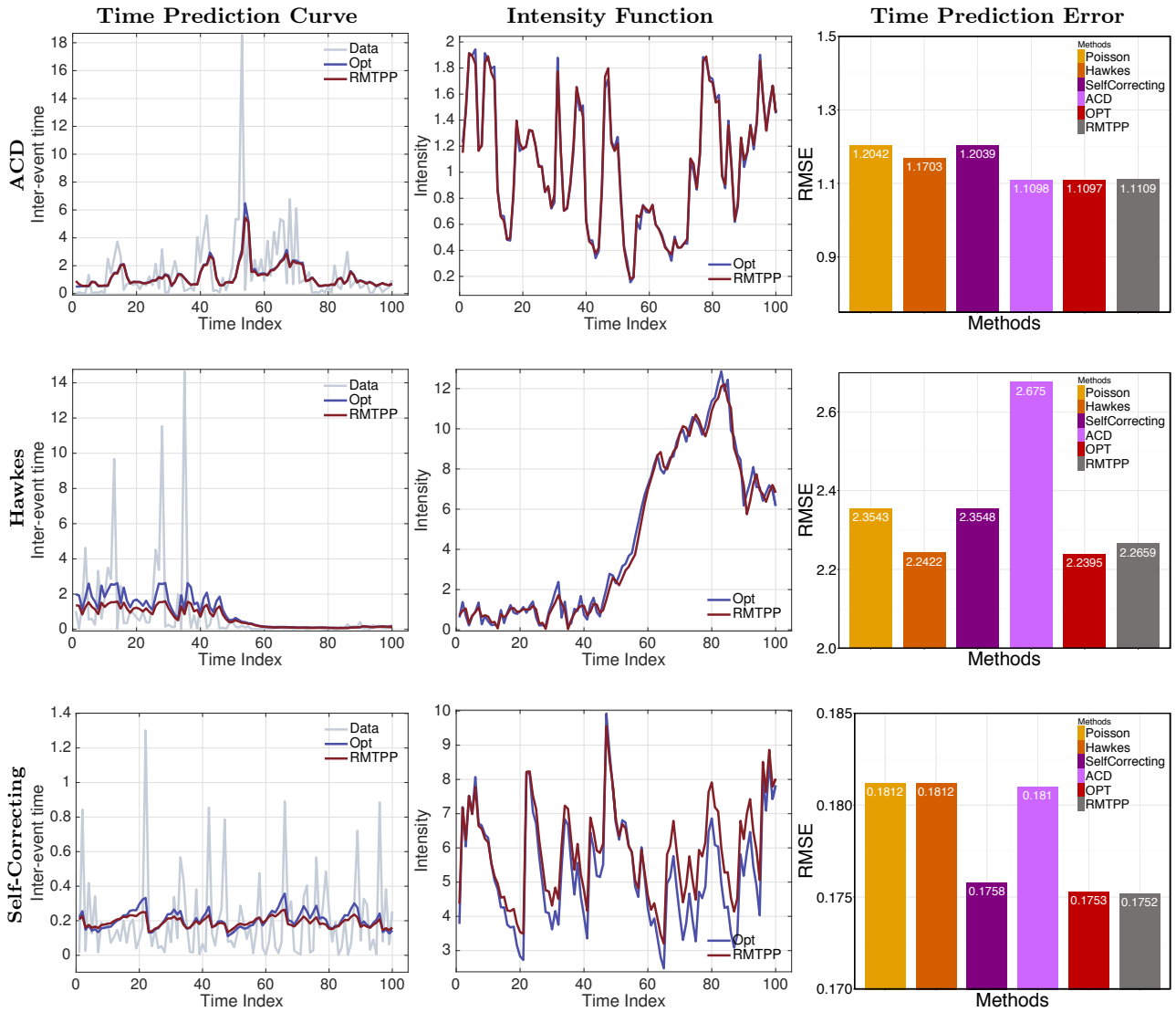
Figure 4: Time predictions on the testing data produced from different processes. Left column is the predicted inter-event time. Blue curve is the optimal estimator, and red curve is RMTPP without any prior knowledge about the true dynamics of each case. Middle column shows the learned intensity functions vs. the respective true ones. Right column gives the overall testing RMSE of predicting the timings from different processes.
