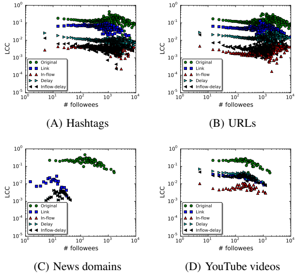
Figure 14: Average local clustering coefficient versus the number of followees in the original ego-network (green circles) and the ego-networks optimized for link (blue squares), in-flow (red triangles), delay (teal triangles), and inflow-delay efficiency (black triangles).
