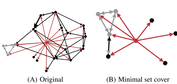
Figure 12: Ego-networks for a Twitter user (red node). Some users (black nodes) only belong to one of the ego-networks while others (gray nodes) belong to both. The original ego-network contains more triangles than the ego-network induced by the minimal set cover, whose structure is closer to a star.
