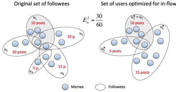
Figure 3: Our notion of in-flow efficiency, E_u^f . We define in-flow efficiency as E_u^f = f(\mathcal{U}^f(\mathcal{I}_u)) / f(\mathcal{U}_f) , where \mathcal{I}_u is the set of (unique) memes (blue circles) a user receives in her timeline by following a set of followers \mathcal{U}_u = \{u_1, \dots, u_5\} (left), and \mathcal{U}^f(\mathcal{I}_u) = \{u_1^*, u_2^*, u_3^*\} (right) is the set cover (of users) with the smallest associated in-flow f(\mathcal{U}^f(\mathcal{I}_u)) that, if followed, would provide the same set of memes \mathcal{I}_u . In the illustration, each user u_i posts the memes within the associated ellipsoid and the red values in the ellipsoid represent the in-flow of each user. Hence, in this case, the in-flow efficiency value is E_u^f = 30/60 = 0.5 .
