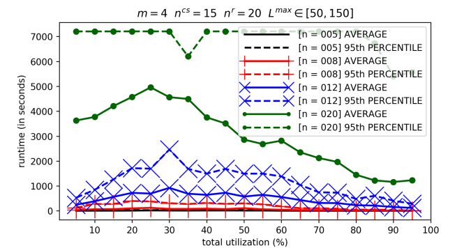
(g) FP-SAG-SR runtime for varying task set size n
