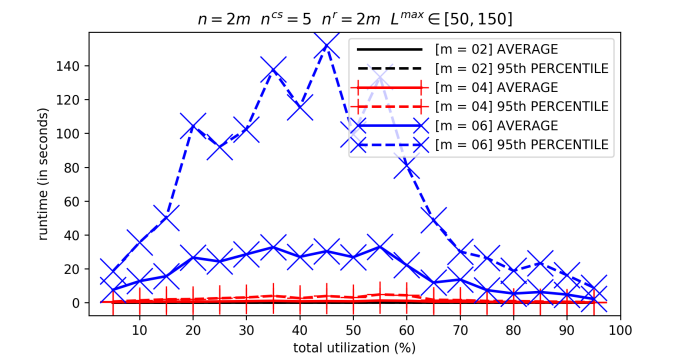
(h) FP-SAG-SR runtime for varying processor count m
