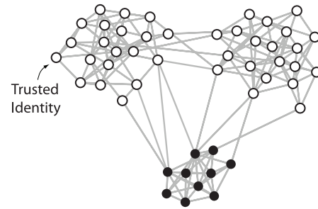
Fig. 3. Non-Sybils are hollow and Sybils filled. The trusted identity cannot distinguish between the non-Sybil community and the Sybil community.
