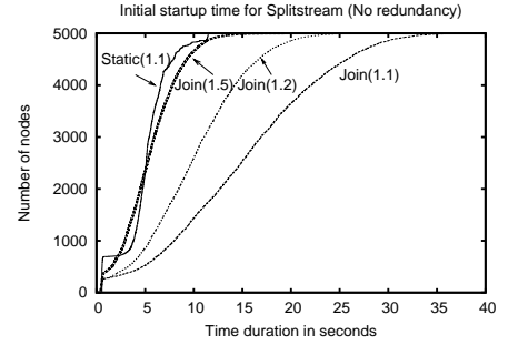
Fig. 7. Initial startup time in Splitstream
