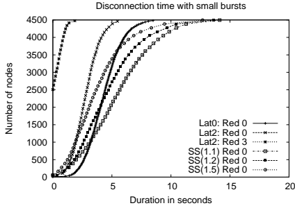
Fig. 11. Recovery duration for 10% burst
