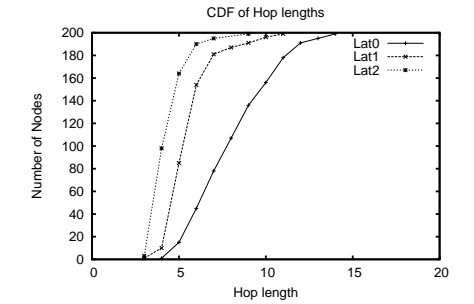
Fig. 16. Emulation result: CDF of Hop lengths
