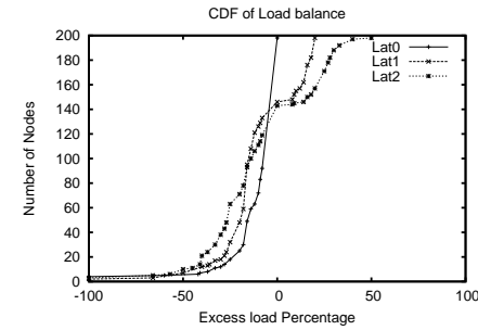
Fig. 15. Emulation result: CDF of Load Distribution
