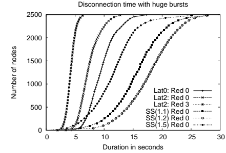
Fig. 12. Recovery duration for 50% burst
