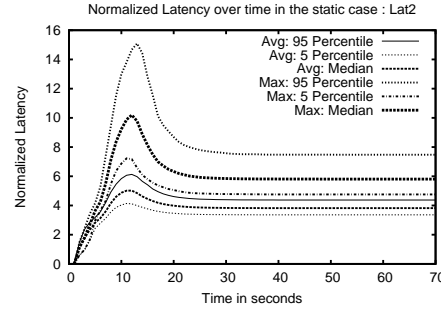
Fig. 9. Maximum and average latencies over the simulation time in the static case
