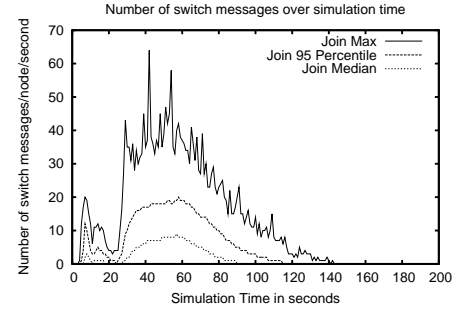
Fig. 10. Control Overhead in Chunkspread: Switch messages over simulation time
