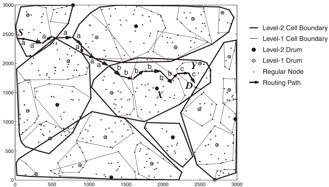
Fig. 1. Masai routing example: A packet from source node S is routed to destination node D
