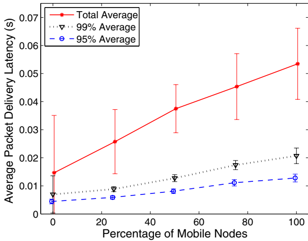
Fig. 11. Average packet delivery latency vs. percentage of mobile nodes in 1000-nodes networks
