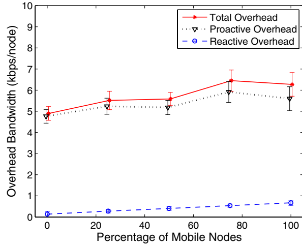
Fig. 10. Overhead bandwidth per node vs. percentage of mobile nodes in 1000-nodes networks
