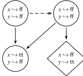
Fig. 3. STS for a Variant of the “Deferred Divergence” Example
