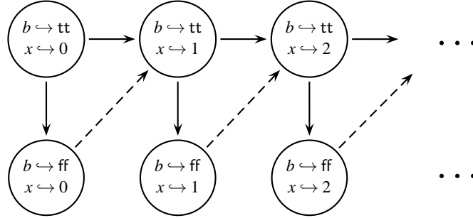
Fig. 2. STS for the “Callback with Lock” Example in HOS
